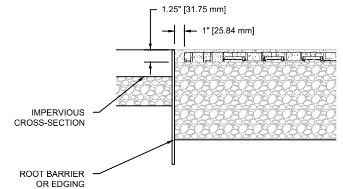
IMPERVIOUS ABUTMENT
