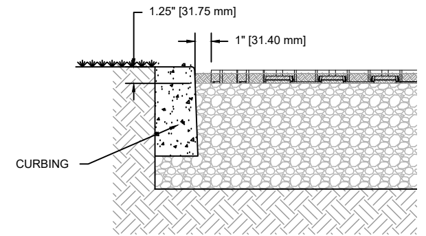
CURB ABUTMENT
